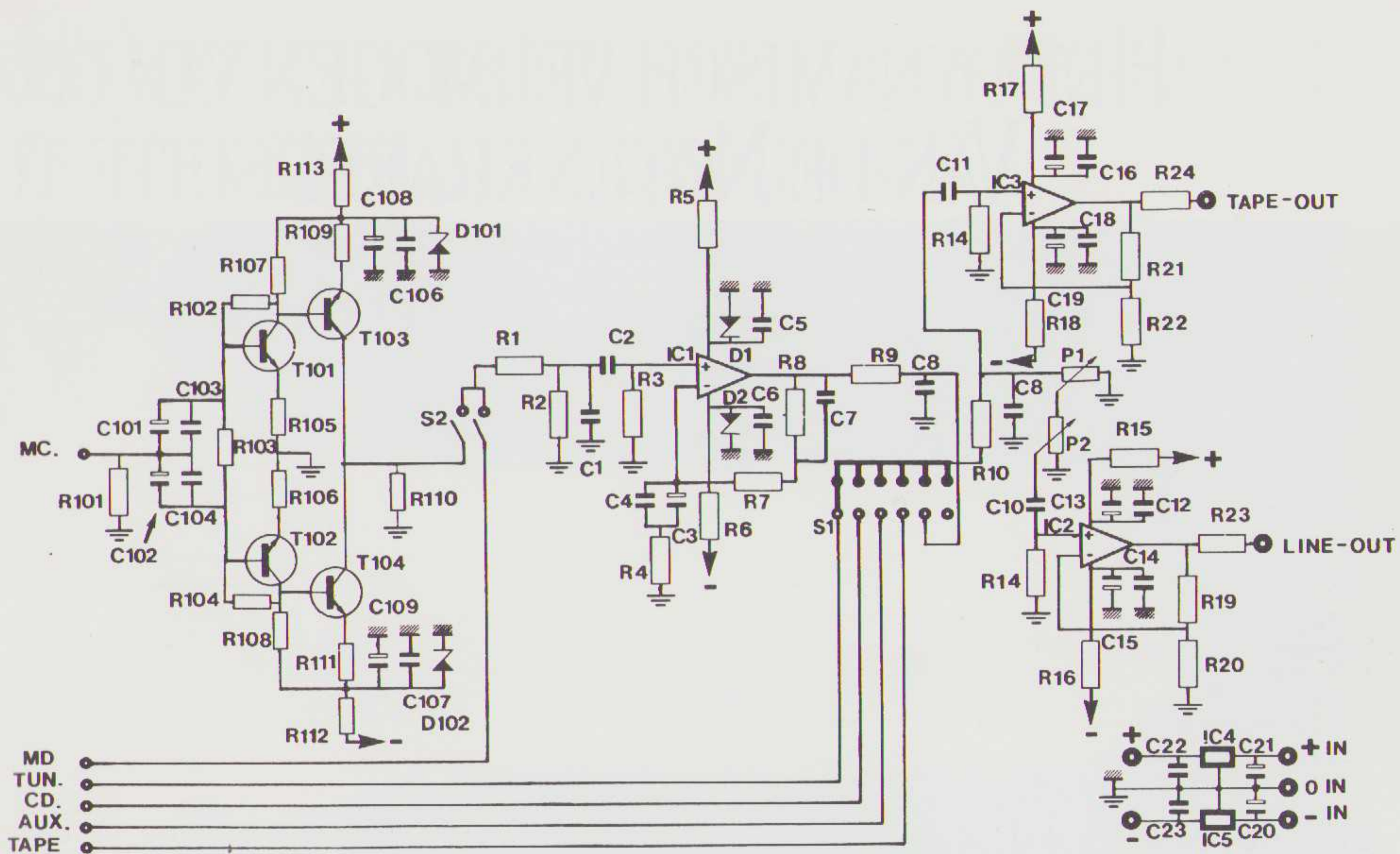
YPSILON P851
